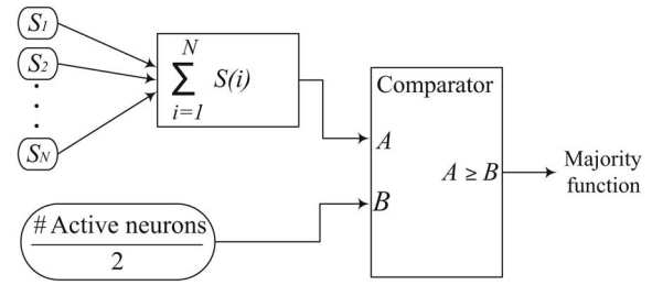
Fig. 3. Functional diagram of the S module for computing the majority function of the hidden neurons outputs.
