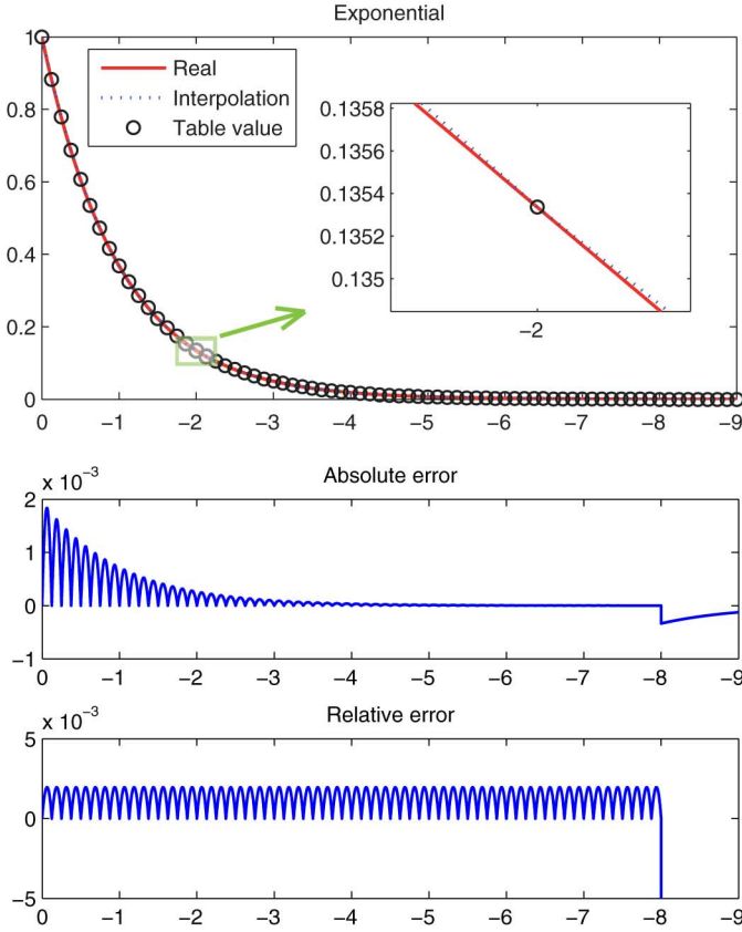
Fig. 5. Exponential function and approximated value (top graph). Absolute (middle) and relative errors (bottom) committed in the approximation of the exponential function (see text for more details).
