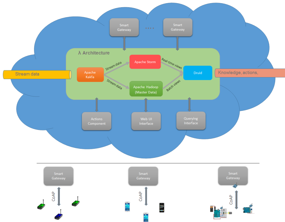
Fig. 1. The \lambda -CoAP Architecture
