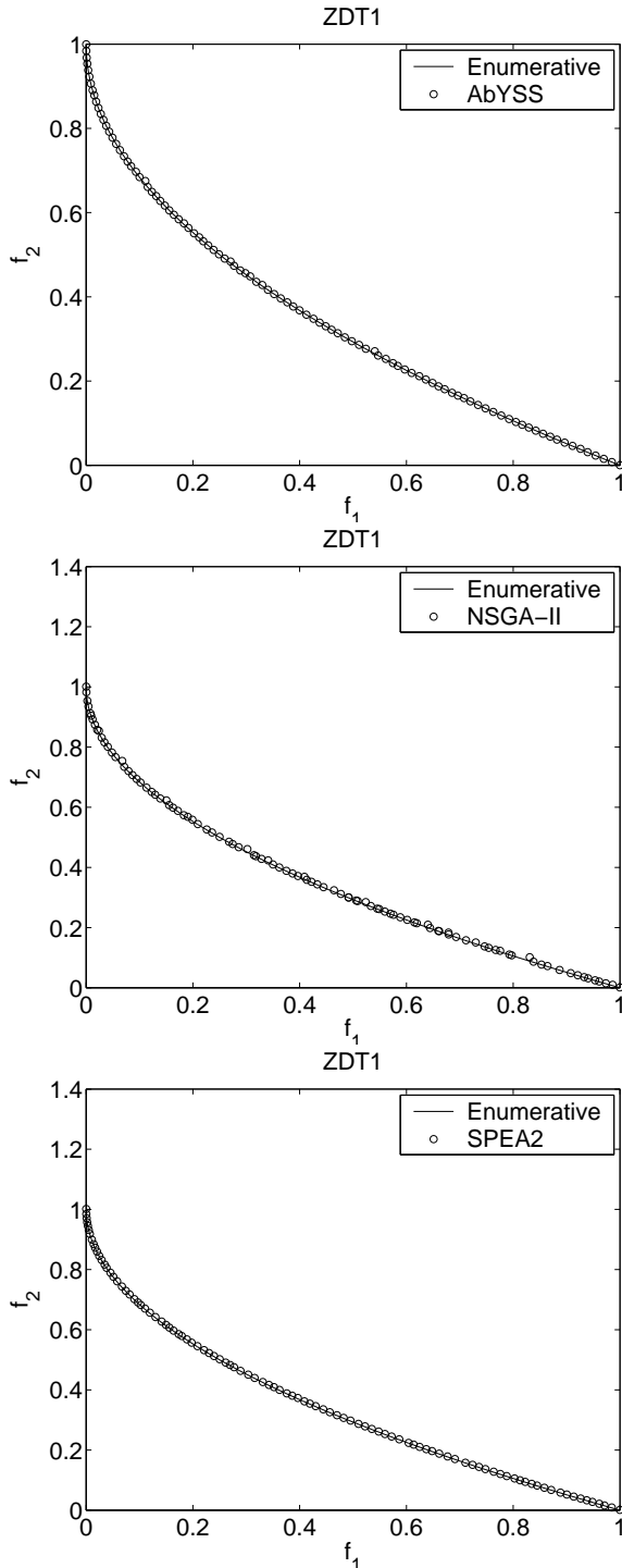
Fig. 9. Pareto fronts obtained with the three algorithms on problem ZDT1.
