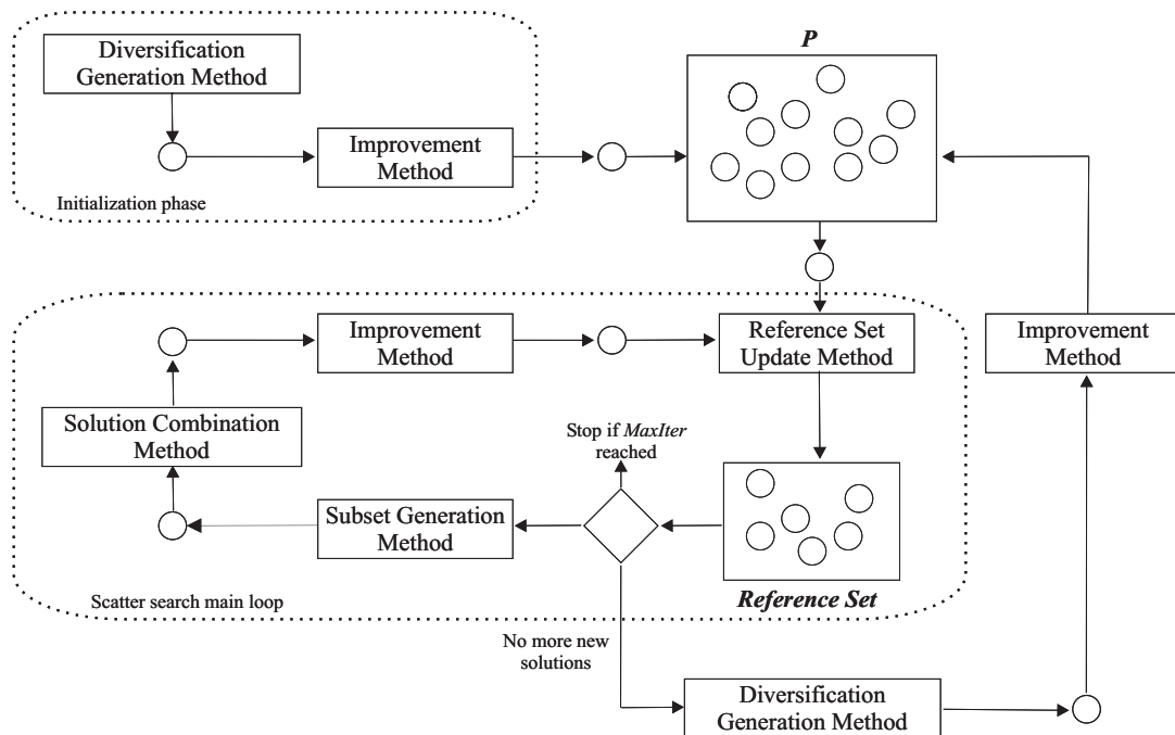
Fig. 1. Outline of the standard scatter search algorithm.
