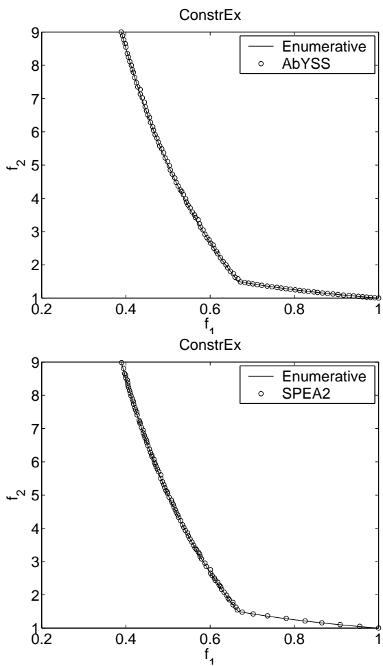
Fig. 11. Pareto fronts of the problem Constr.Ex with AbYSS and SPEA2.
