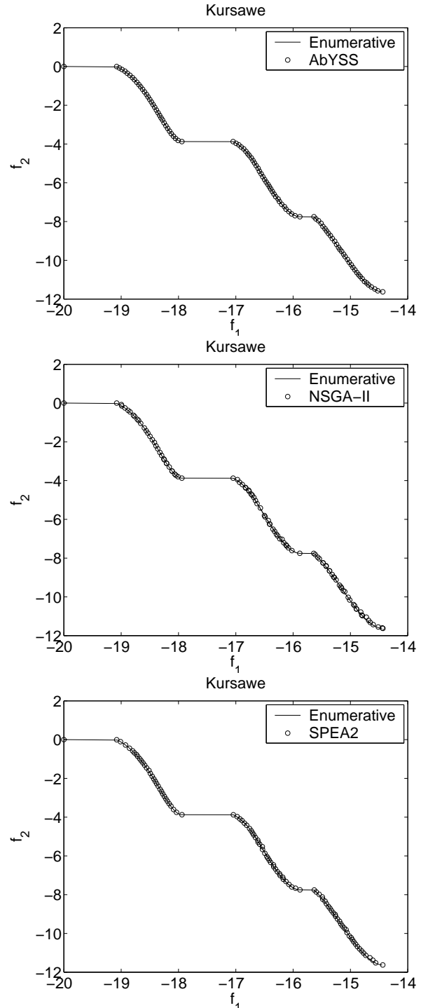
Fig. 8. AbYSS finds a better spread of solutions than SPEA2 and NSGA-II in the Kursawe problem.
