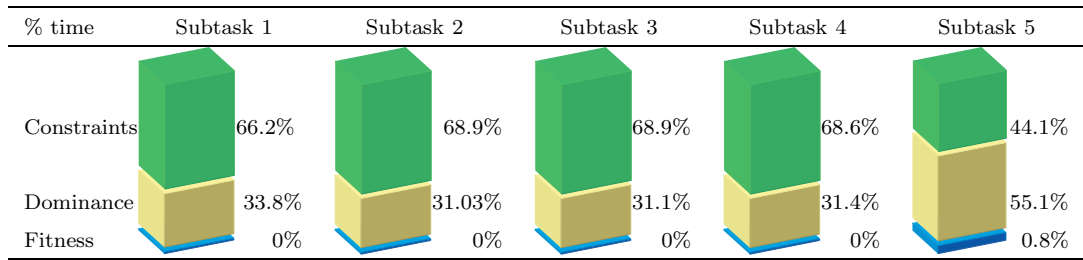
Fig. 7. Percentage of time spent in evaluating the constraints, the dominance tests, and the fitness function for the problem Golinski.
