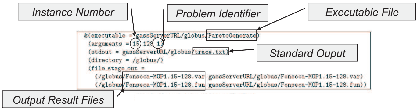
Fig. 2. Example of an RSL specification.
