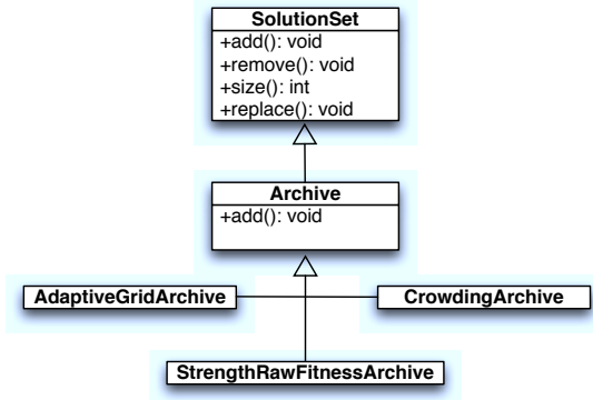
Fig. 6. Archives included in jMetal.
