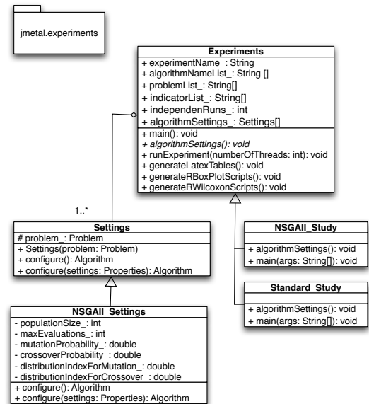
Fig. 8. Classes and their relationships in the jmetal.experiments package.
