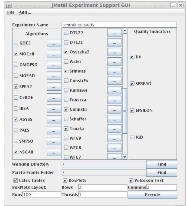
Fig. 9. Configuring an experiment with the GUI tool.
