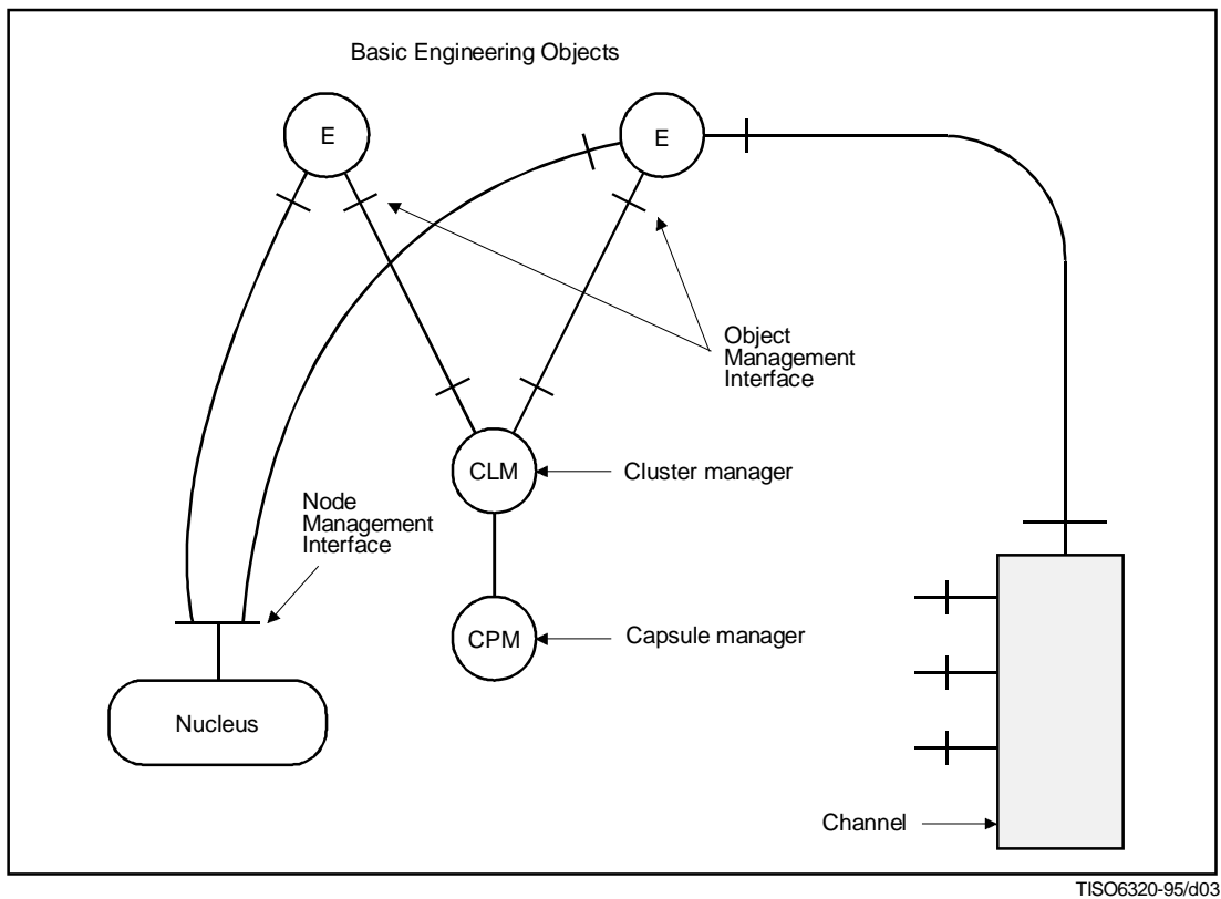
Figure 4 – Example structure supporting a basic engineering object
