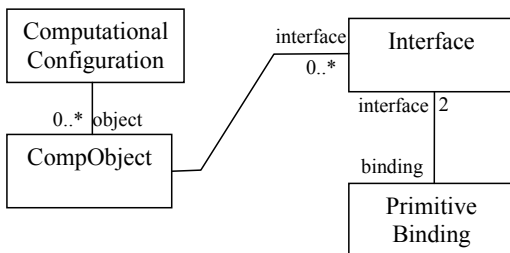
Figure 2 Computational Objects
