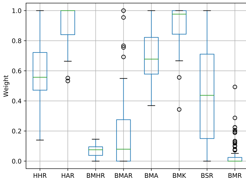
Figure 6: Boxplots of the weight distribution that score the changes on the battlefield (the ones shown in Table 1 used to calculate \Delta_{attributes(hero)}^{a,S} , \Delta_{minions(hero)}^{a,S} , \Delta_{secrets(hero)}^{a,S} and \Delta_{manaConsumed}^{a,S} . These weight distributions have been obtained from all the individuals of the last generation of all runs.
