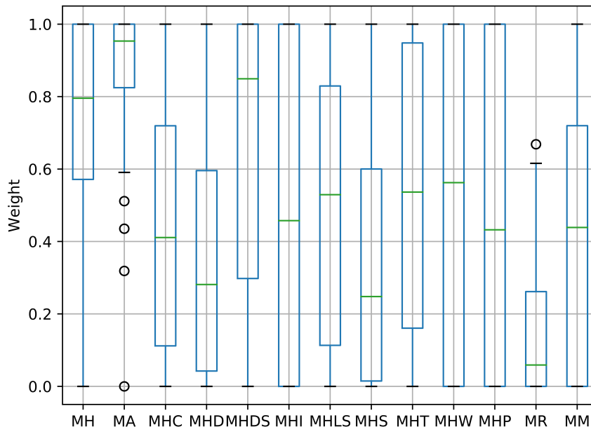
Figure 7: Boxplots of the distributions of those weights that score a minion via the function valueOf(m) and that are shown in Table 2. These distributions have been obtained from the 100 individuals at the end of all runs ( \mu \cdot E = 10 \cdot 10 ).
