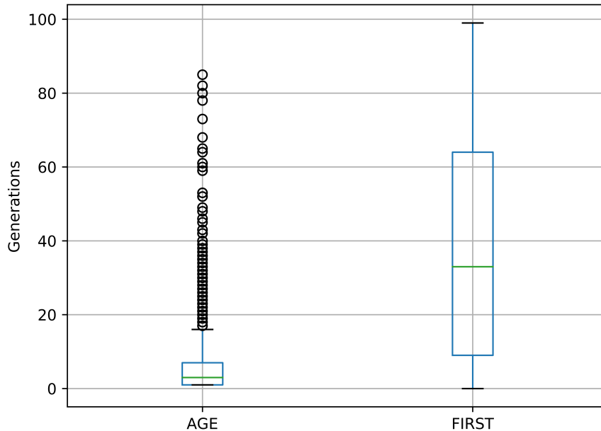
Figure 3: Boxplots describing individuals' lifespan over all the 10 ( E ) runs. ( AGE ) describes the age of all individuals produced and ( FIRST ) shows the first generation that an individual entered the main population, thus being able to defeat at the very least the weakest individual in the previous population
