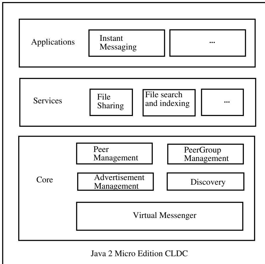
Fig. 4. JMobiPeer Architecture
