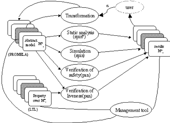
Fig. 1. Overview of an environment for verifying by transformation
