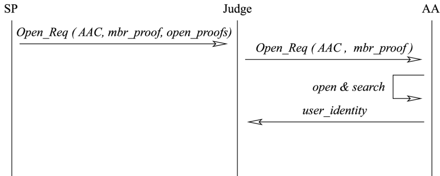
Figure 10. Disclosing user's identity
