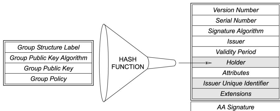
Figure 2. Anonymous attribute certificate
