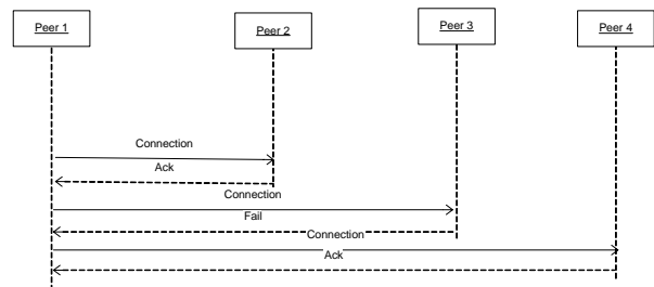
Fig. 7. Sequence diagram: Discovery phase
