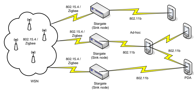
Fig. 4. Prototype layout
