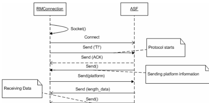
Fig. 6. SerialForwarder connection protocol
