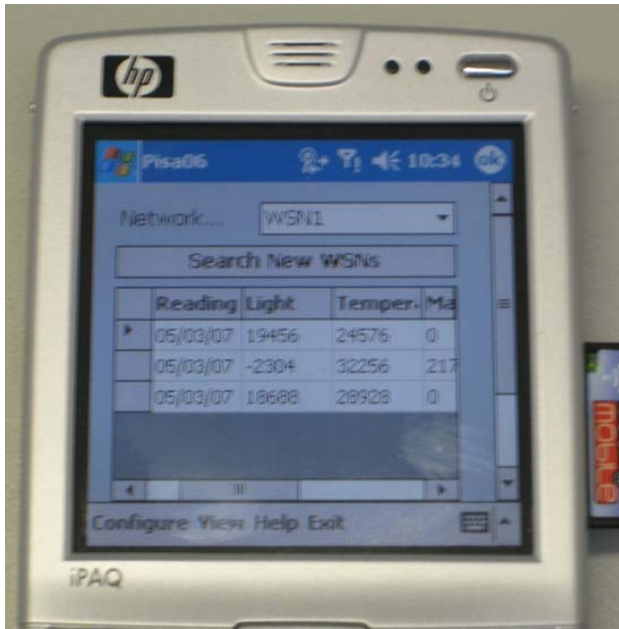
Fig. 5. Front-end application
