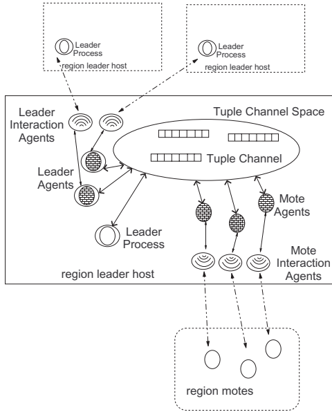
Figure 4. Middleware architecture.
