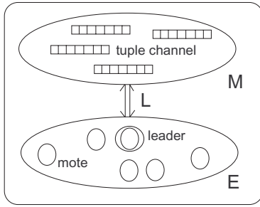
Figure 2. Virtual Machine.
